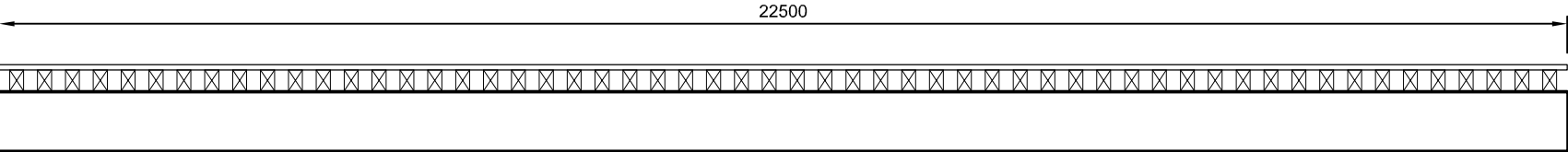
ELEVATION 1:100 GIRDER
