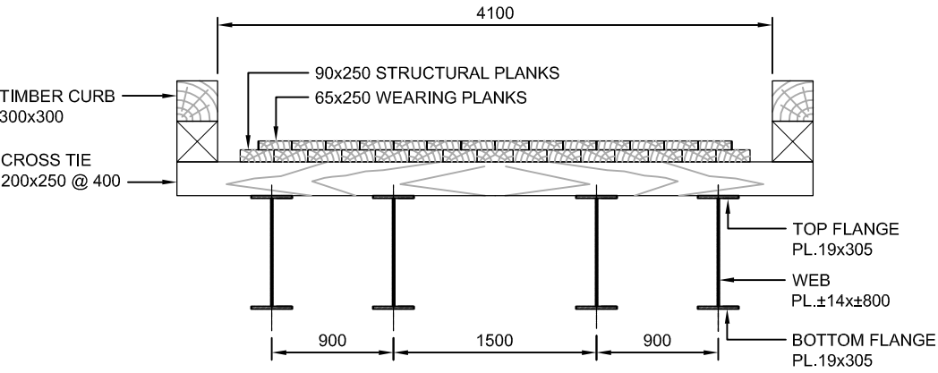
TYPICAL SECTION
